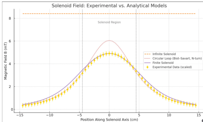
Figure 7: The magnetic field against position data compared against three models that are based on various solenoid shapes. Grey, vertical lines represent the length of the solenoid. The best fitting model is the finite solenoid model, showing a gradual drop-off of the field which better matches the experimental data. Graph was made with current 0.48 amps, not 0.20 amps.
