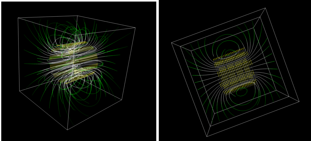
Figure 1: Simulated magnetic fields of a solenoid. On the left is a three dimensional view of the fields, on the right is a slice of the X Plane. The field lines shown on the right give a clear view of the magnetic field on the inside of a short solenoid.
