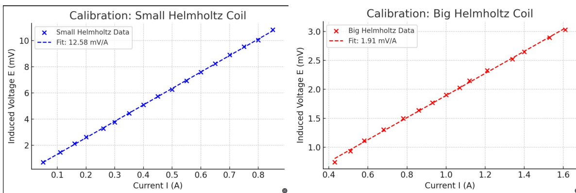
Figure 5: Calibration graphs relating induced voltage to current in a pair of Helmholtz coils. The graph on the left is from the Eisco model Helmholtz coils, and the curve fits very well. The graph on the right is from the Leybold model Helmholtz coil. The curve does not fit as well as the Leybold model is an older design that produces significantly smaller voltages.
