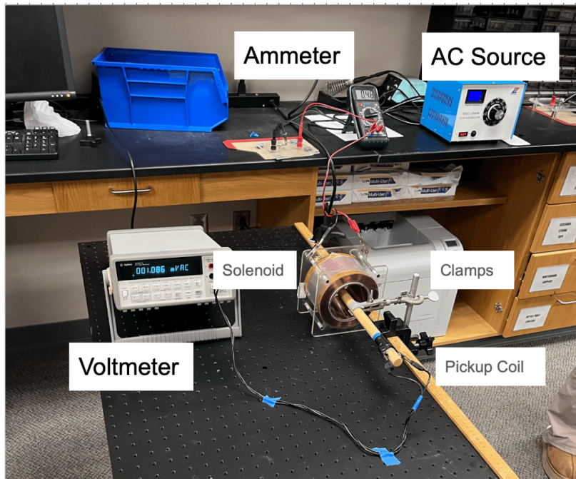
Figure 4: Experimental setup for solenoid field mapping.
