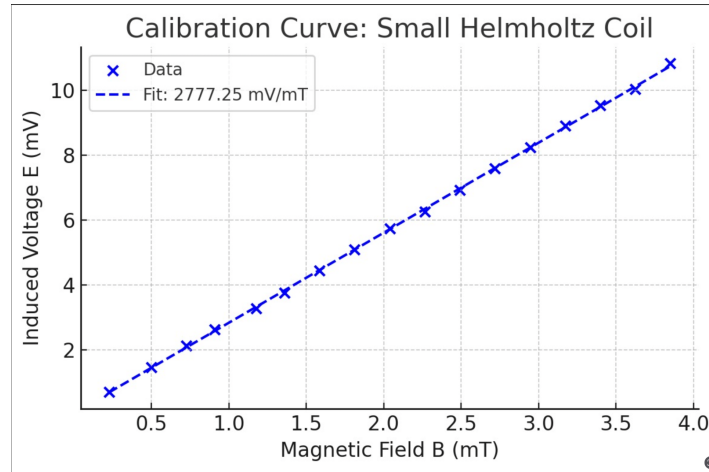
Figure 6: Eisco model Helmholtz coil final calibrated curve relating induced voltage to the magnetic field. This is the chosen calibration used for the data from the pickup coil.
