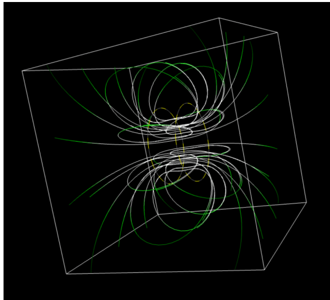
Figure 2: Simulated magnetic field between Helmholtz coils separated by their approximate radius. This shows the uniform nature of Helmholtz coils in this configuration.
